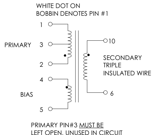
FIGURE 1: SCHEMATIC DIAGRAM
